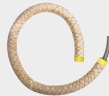
490-04 Seepage hose for Hawle underground hydrants
