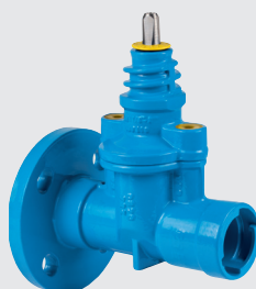
255-00G Service valve for gas with ZAK ® socket and flange
