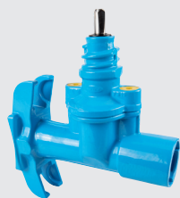
270-01G Valve saddle with ZAK® outlet for gas
