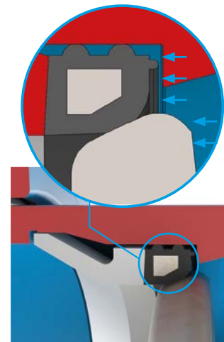
Functional principle 2
