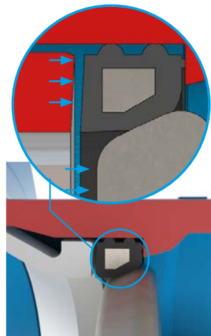
Functional principle 1
