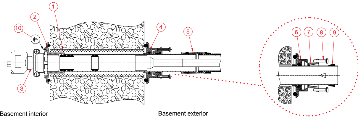
Example of installation of broken masonry with construction tube
